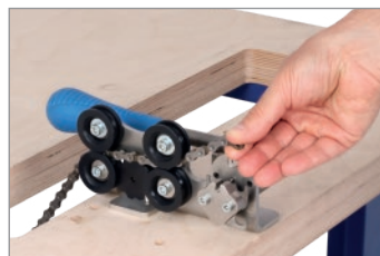
Thread the chain through the tool position first link on rivet pin
